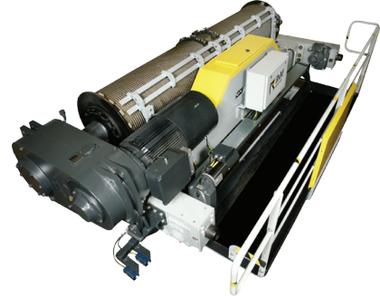
SXL Heavy Lifting Winch 10-250 Ton Capacity
