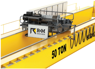
DXW Heavy-Duty Hoist 6.3 - 160 Ton Capacity
